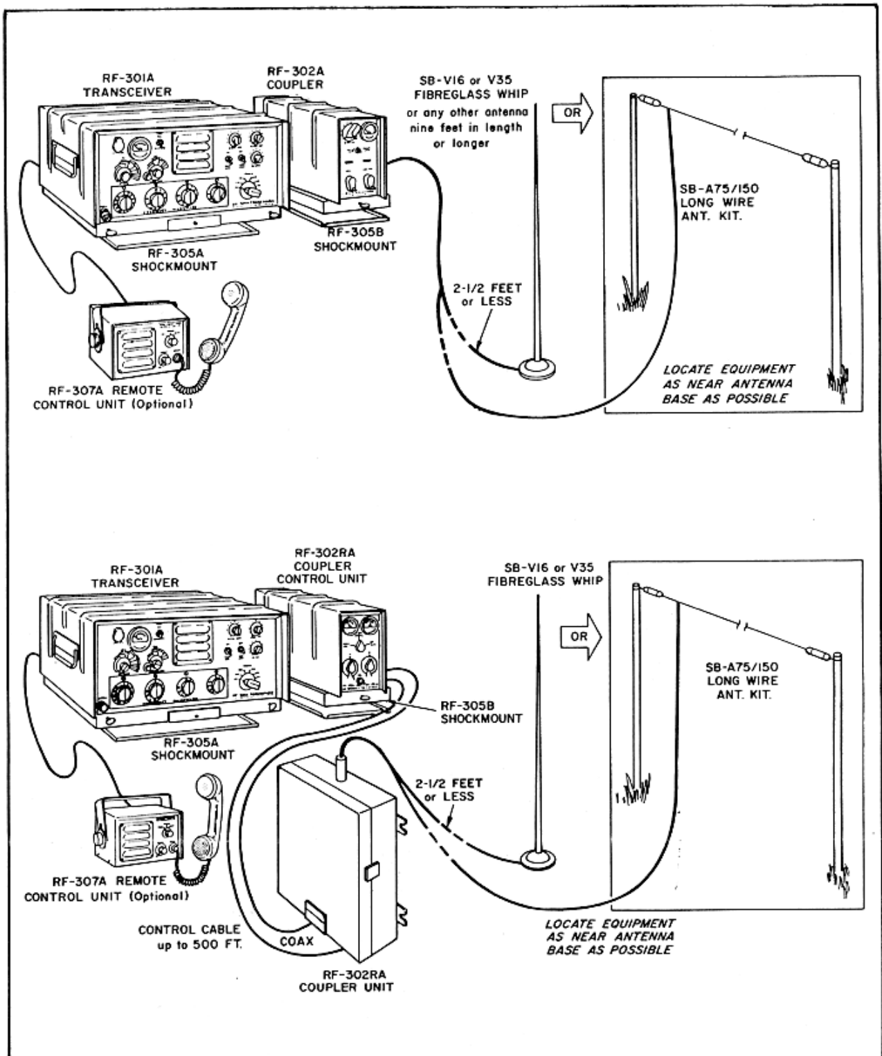
Figure 2.4 – Typical Base Station Installations
