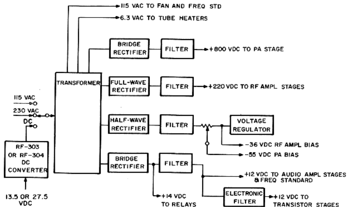
Figure 4.4 - Power Supply Block Diagram
