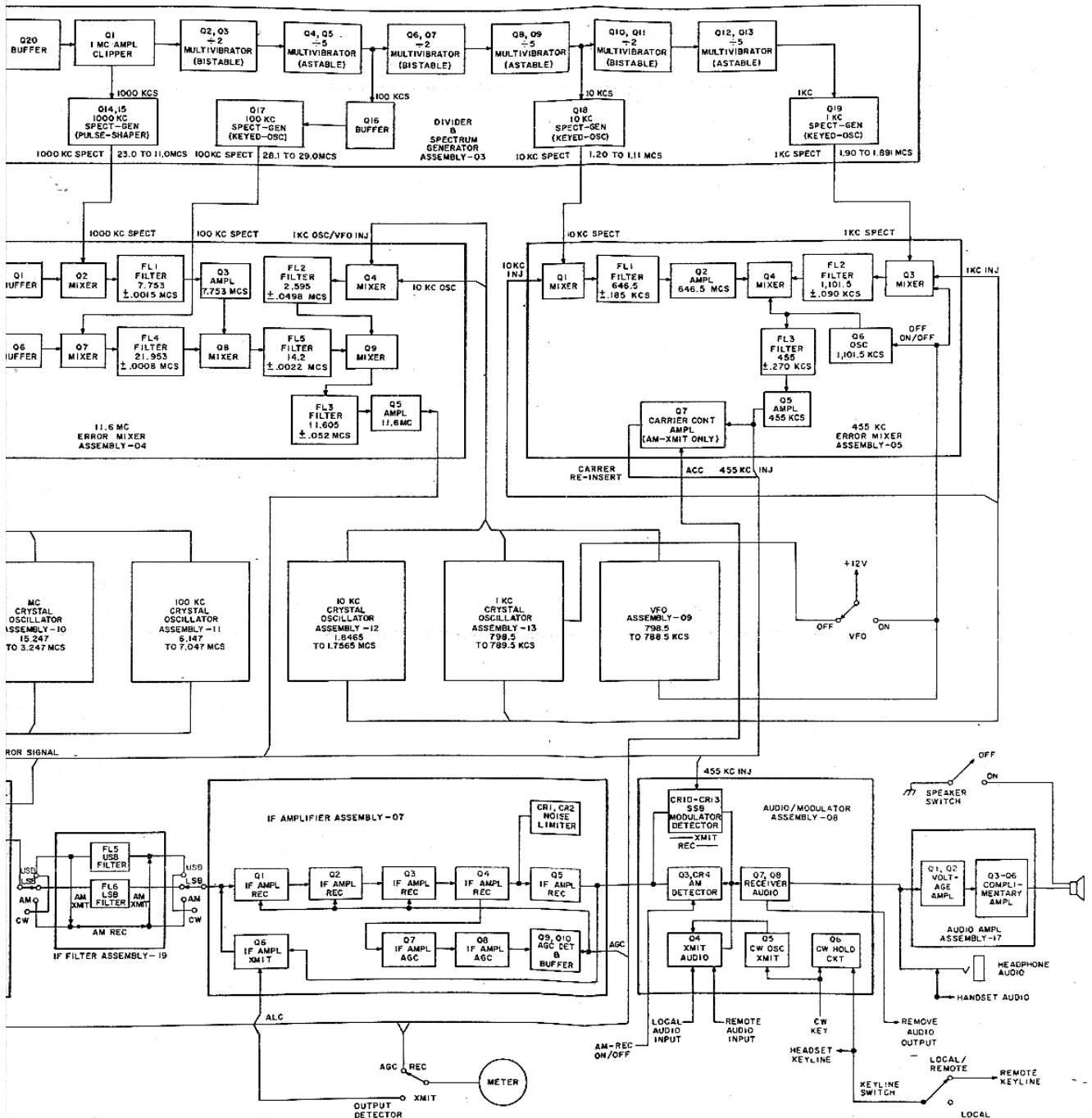
Figure 4.6 – RF-301 Signal Block Diagram
