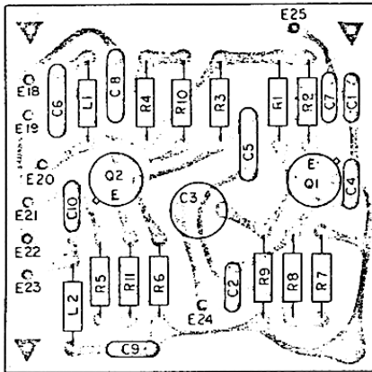
FIG 8.19 100KHZ OSC. PARTS LOCATION
