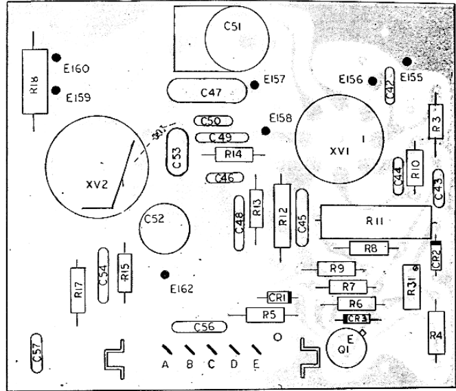
RF Amplifier (162-0260)
