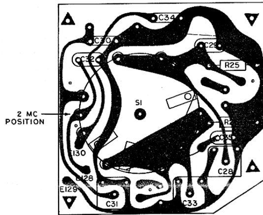
Bandswitch – Sect. D (162-0209)
