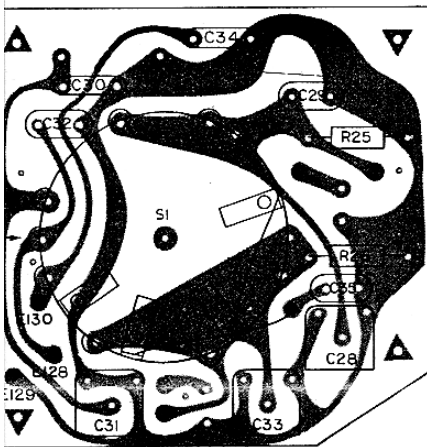
Bandswitch – Sect. D (162-0209)
