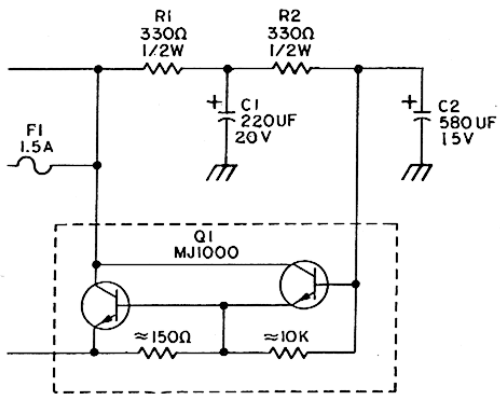
TRANSISTOR FILTER ASSEMBLY
