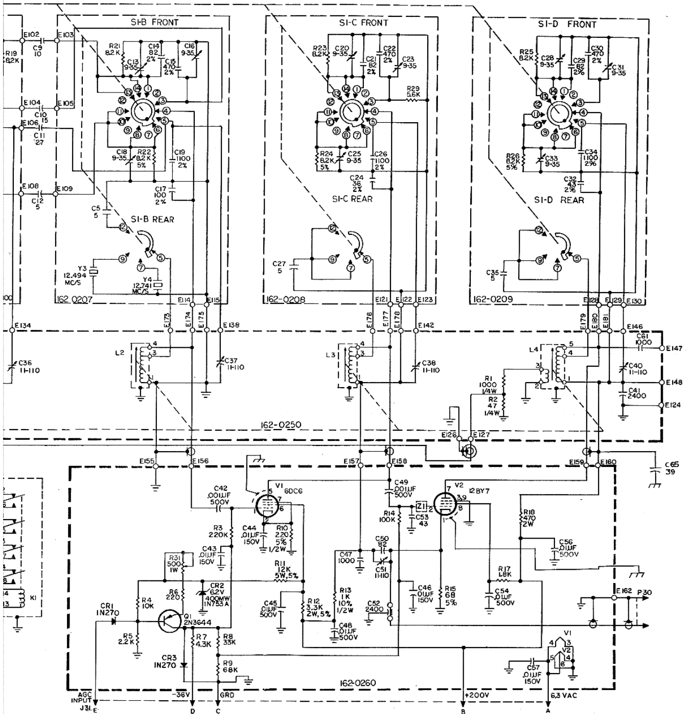
Figure 8.2 – RF Amplifier Schematic Diagram
