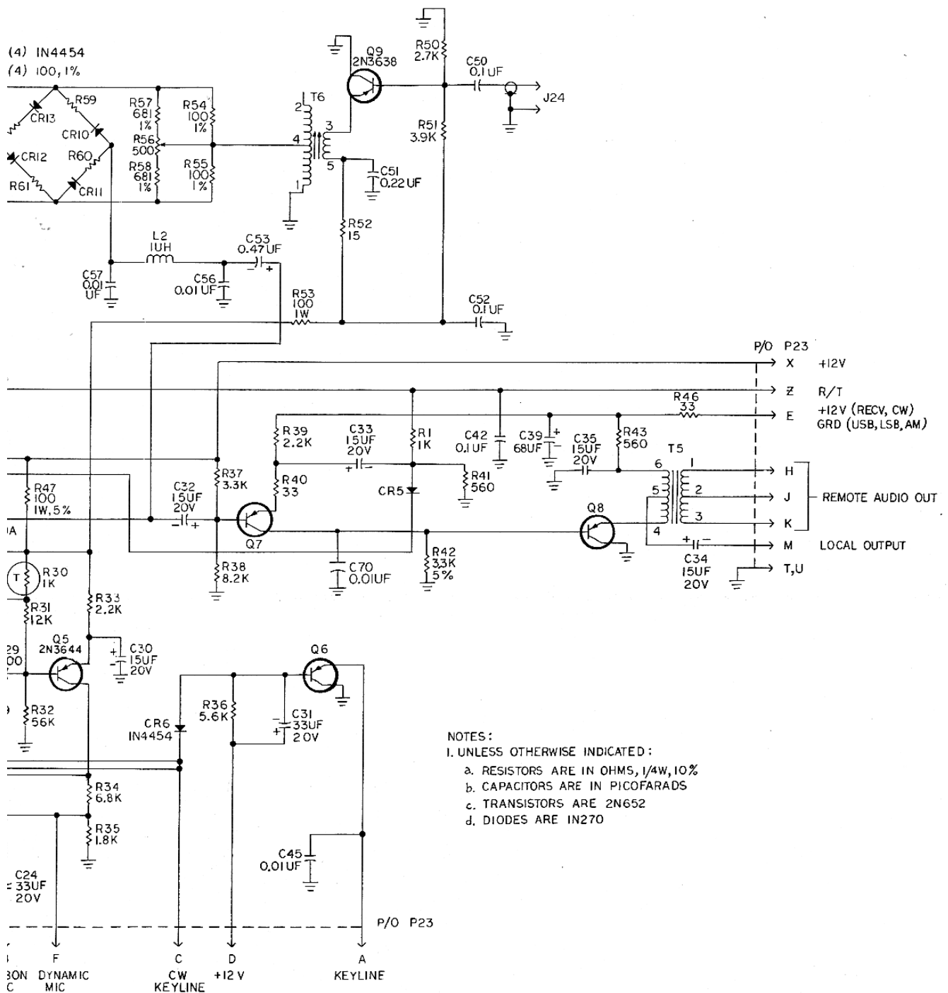
Figure 8.14 – Audio/Modulator Schematic Diagram
