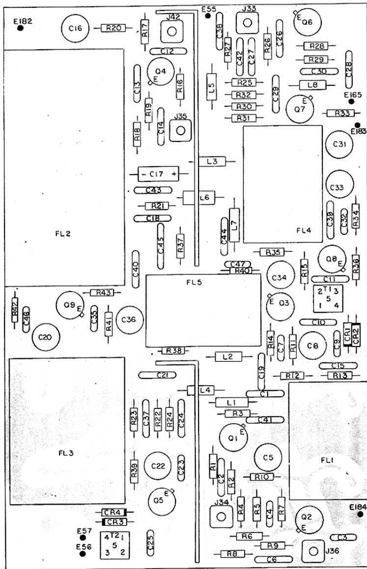
Figure 8.5 11,6 Mhz Error Mixer Parts Location.
