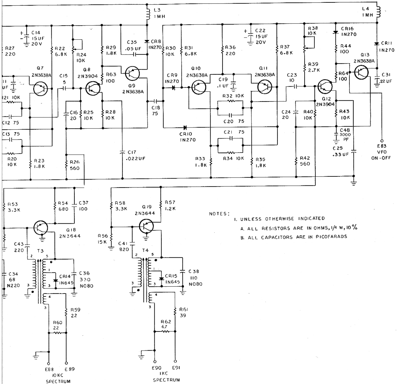
Figure 8.4 – Divider/Spectrum Generator Schematic Diagram
