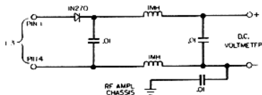
Figure 6.5 — Feedback Detector Test Circuit
