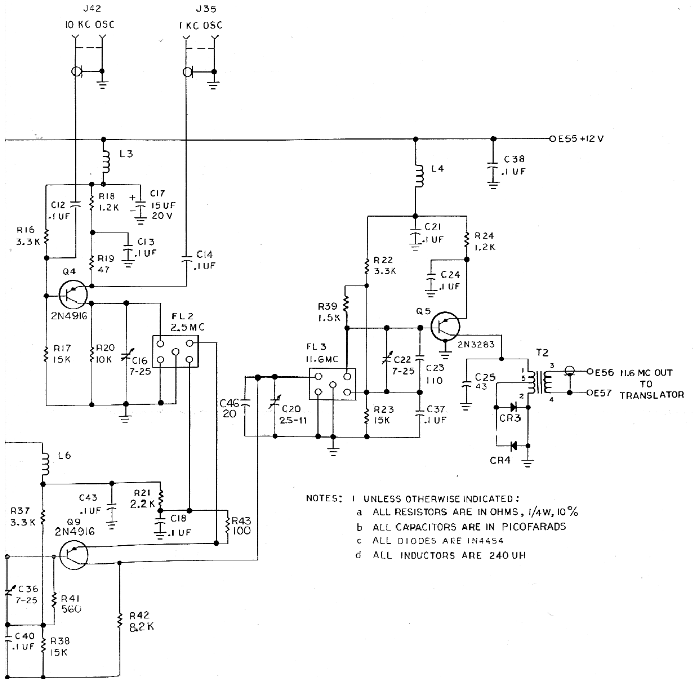
Figure 8.6 — 11.6 MHz Error Mixer Schematic Diagram
