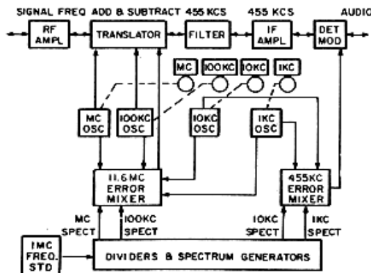
Figure 4.3 – Frequency Synthesizer Block Diagram, Illustrating Signal Flow
