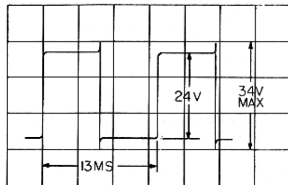
RF-303, 12 VDC Q1 or Q2, Collector
