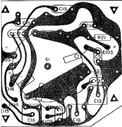
Bandswitch – Sect. B (162-0207)
