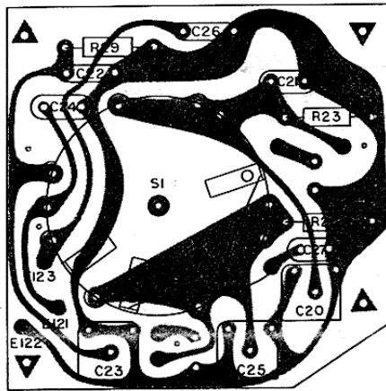
Bandswitch – Sect. C (162-0208)
