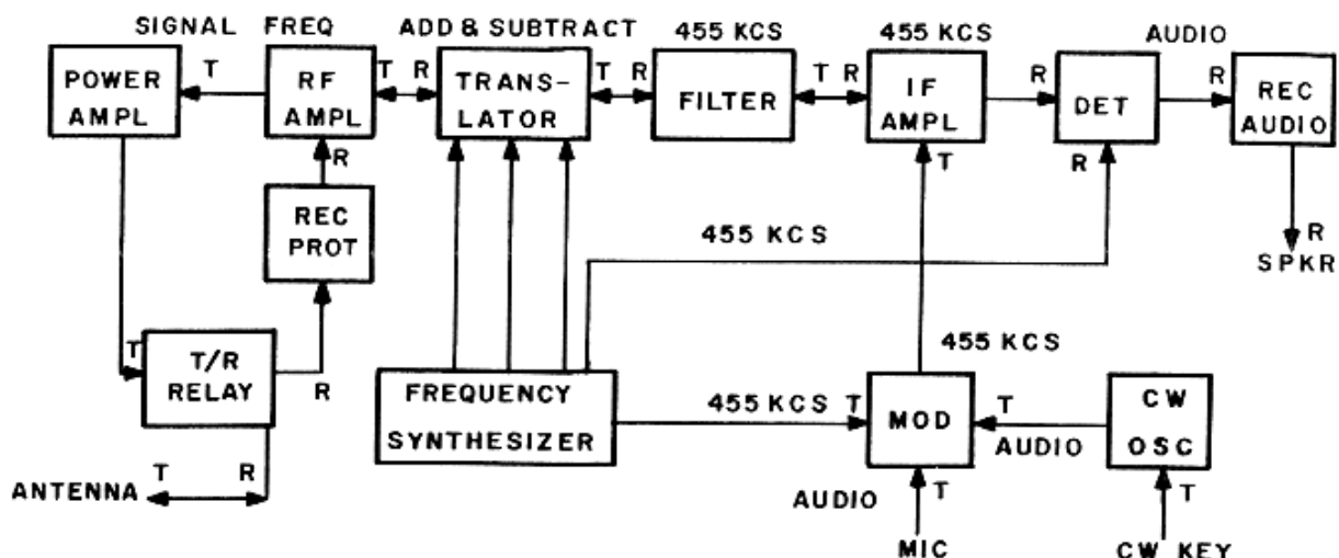
Figure 4.1 — RF-301 Simplified Block Diagram, Illustrating Signal Flow
