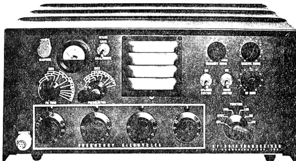
Figure 3.1 – Front Panel Operating Controls
