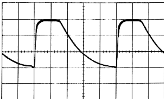
Figure 6.8A – Q1, Base Waveform
