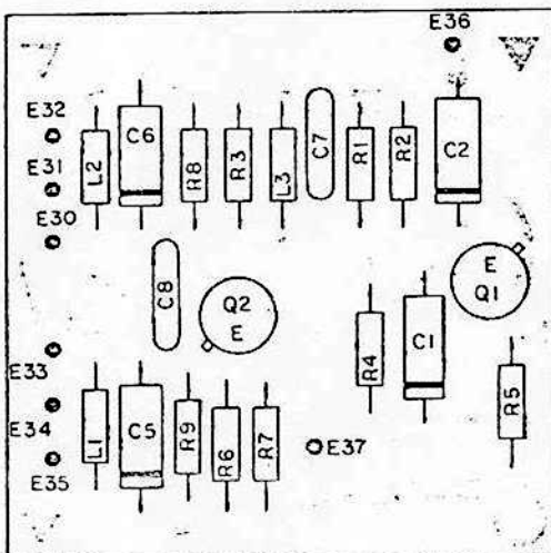
Figure 8.21 – 10 kHz Oscillator Parts Location
