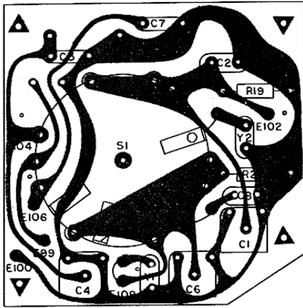
Bandswitch – Sect. A (162-0206)
