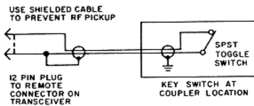
Figure 2.5 – Dummy Load and Key Switches
