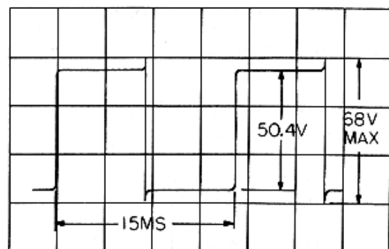
RF-304, 24 VDC Q1 or Q2, Collector
