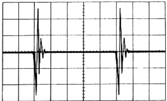
Figure 6.10 – Terminal E84 Waveform
